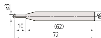
3) 957262 ø3 mm ball (coaxial type)
