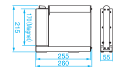
● Dimensions Base (Units:mm)
