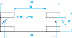
•Dimensions Base (Units:mm)
