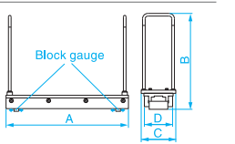
● Dimensions Base (Units:mm)
