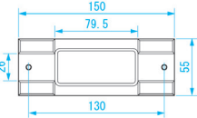
•Dimensions Base (Units:mm)
