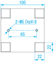
•Dimensions Base (Units:mm)
